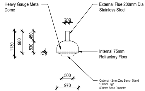
Giotto Rear/Side Elevation
